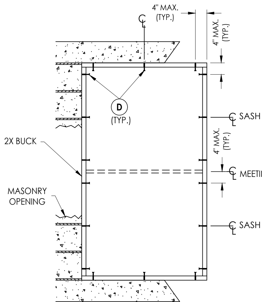
BUCK ANCHORING
