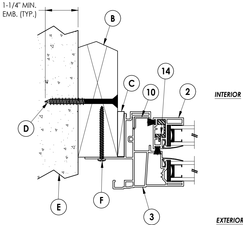
1 HORIZONTAL CROSS SECTION 2x Buck Construction
